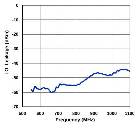
LO Leakage at RF Port
