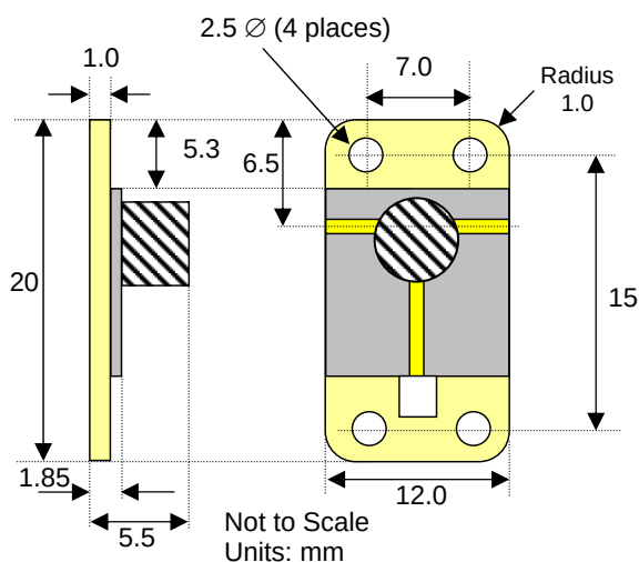
Cross section of the -61 isolator:
