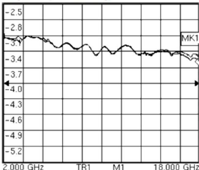
Amplitude (2% Smoothing)
