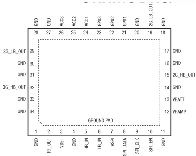
Figure 2. SKY77604 Pad Configuration
