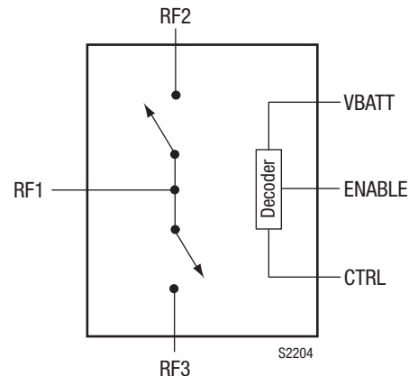
Figure 1. SKYA21003 Block Diagram
