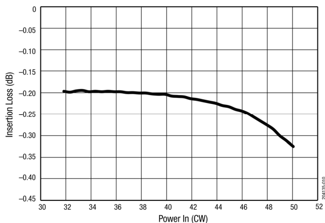
Figure 10. Insertion Loss vs CW Input Power (ANT to TX Port, f = 2.4\text{ GHz} )
