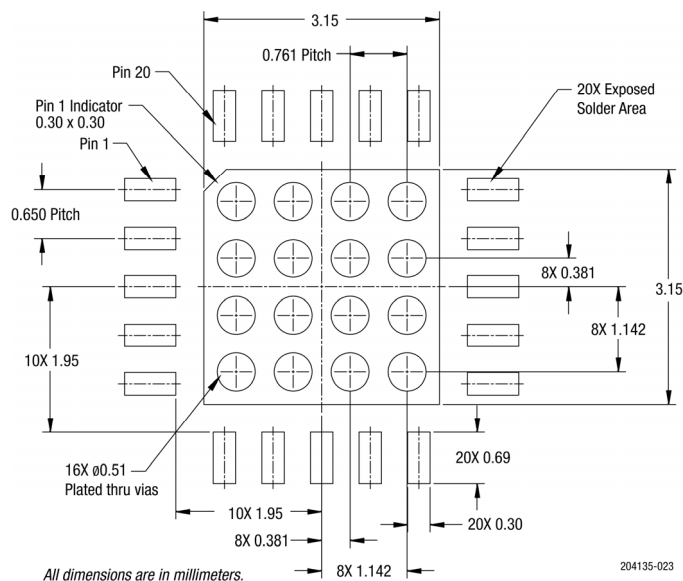
Figure 23. PCB Layout Footprint
