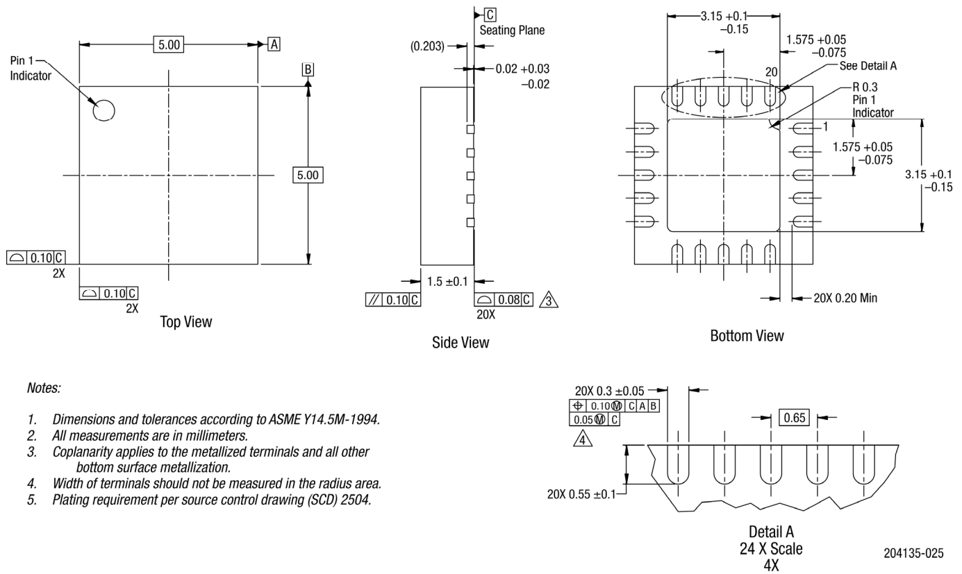
Figure 25. SKY12245-492LF Package Dimensions
