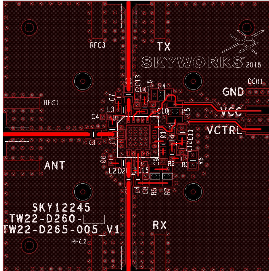
Figure 21. SKY12245-492LF Evaluation Board Assembly Diagram
