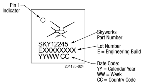
Figure 24. Typical Part Markings (Top View)
