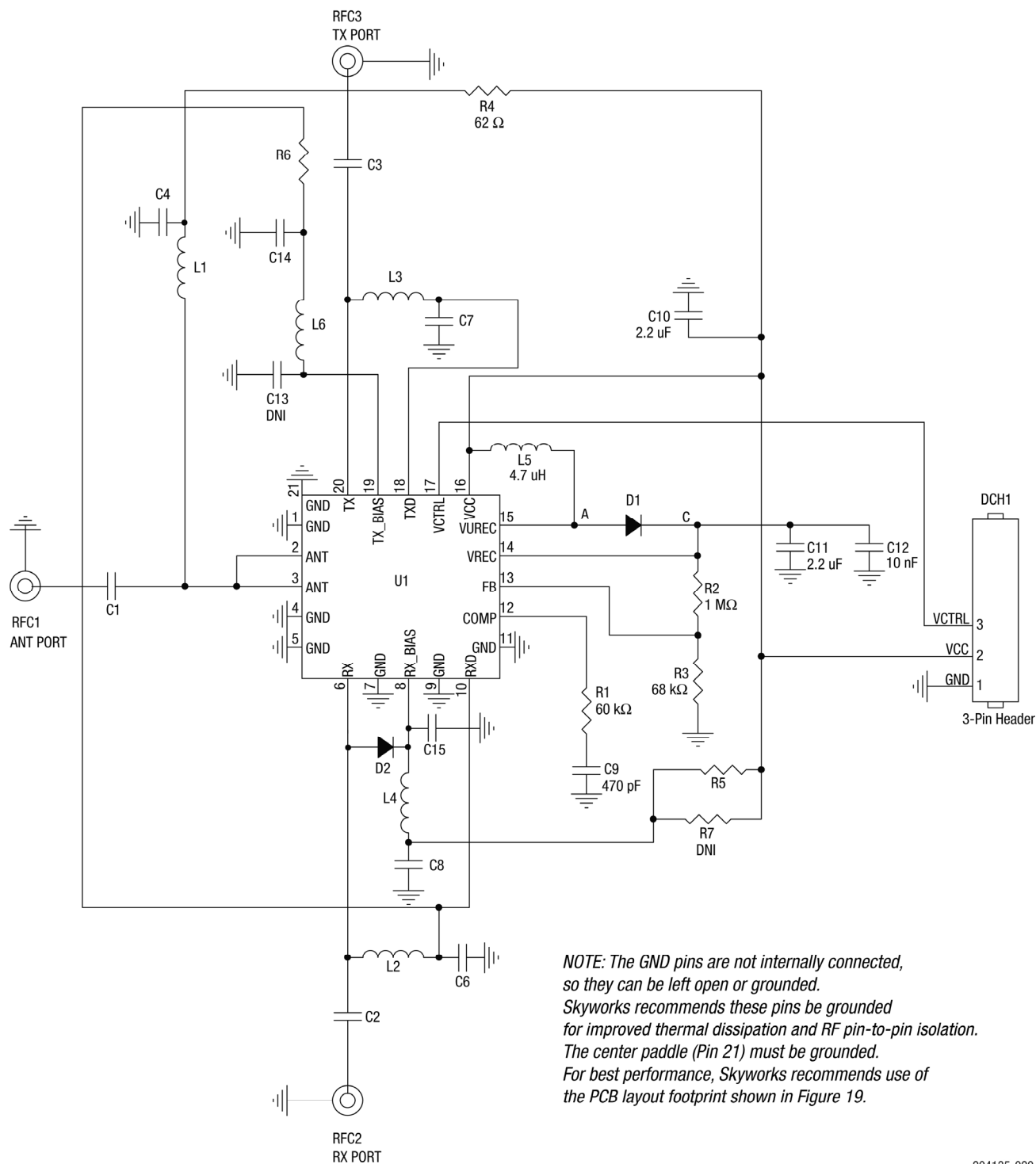
Figure 20. SKY12245-492LF Evaluation Board Schematic
