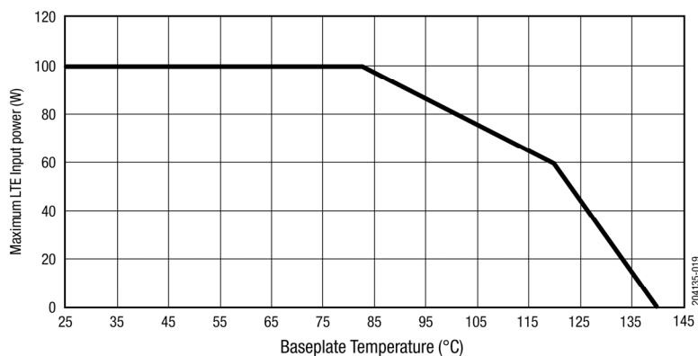
Figure 19. Transmit Power Derating, Maximum LTE Signal Power vs Baseplate Temperature (0.3 dB Insertion Loss)
