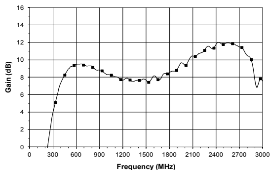
Figure 30: Gain vs. Frequency
