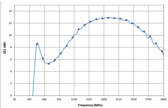
Figure 26: Gain vs. Frequency (V SUPPLY = +9 VDC, 2100 MHz Application Circuit)
