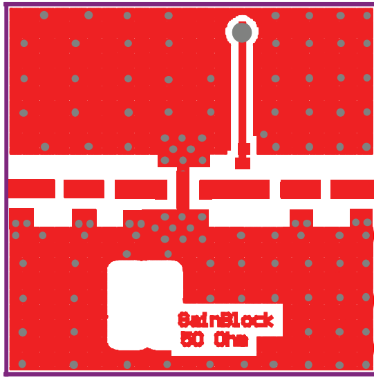
Figure 38: Evaluation Board - Front (not to scale)
