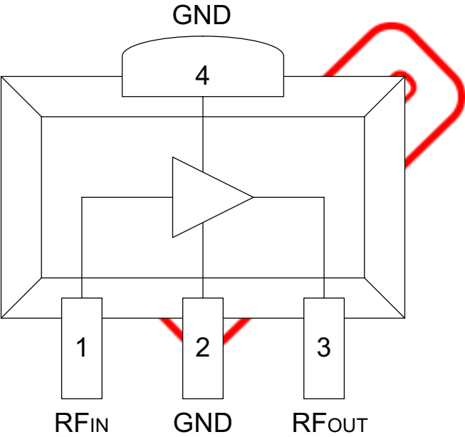
Figure 2: Pin Out
