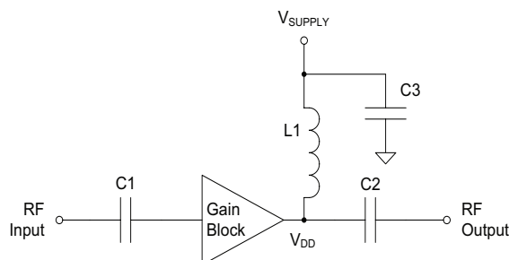
Figure 36: Unmatched Bias Circuit
