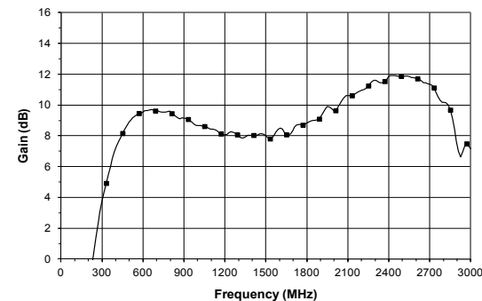
Figure 34: Gain vs. Frequency (V SUPPLY = +5 VDC, 2500 MHz Application Circuit)
