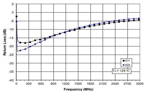
Figure 8: Return Loss vs. Frequency (in Unmatched 50\Omega Test Circuit)
