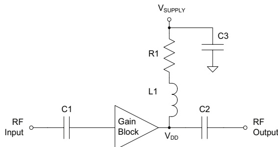
Figure 37: Bias Circuit with Optional Feedback/Voltage Drop Resistor
