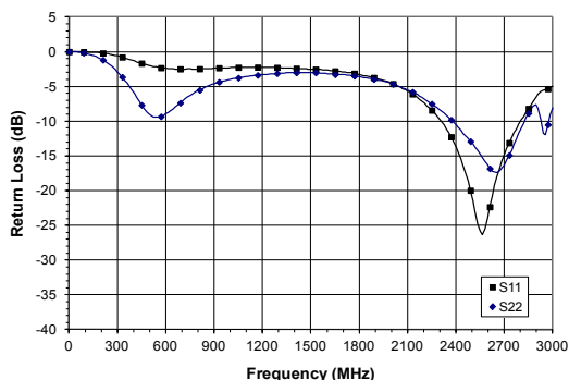
Figure 31: Return Loss vs. Frequency
