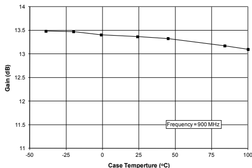
Figure 7: Gain vs. Case Temperature (in Unmatched 50\Omega Test Circuit)
