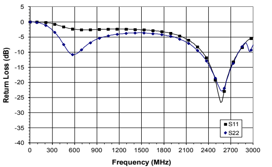
Figure 35: Return Loss vs. Frequency (V SUPPLY = +5 VDC, 2500 MHz Application Circuit)
