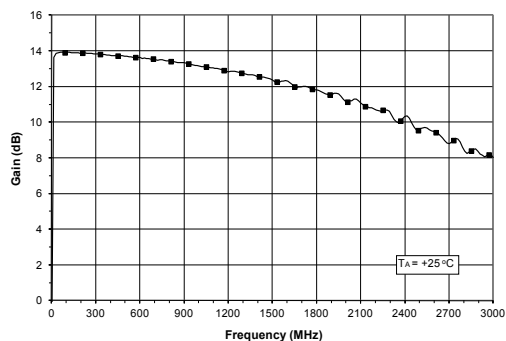
Figure 6: Gain vs. Frequency (in Unmatched 50\Omega Test Circuit)
