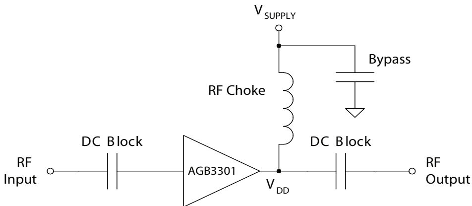
Figure 3: Unmatched 50 \Omega Test Circuit
