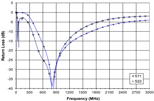
Figure 16: Return Loss vs. Frequency
