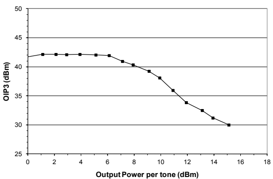
Figure 33: Output 3rd-Order Intercept vs. Power (V SUPPLY = +5 VDC, 2500 MHz Application Circuit)
