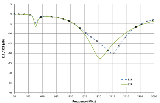
Figure 27: Return Loss vs. Frequency (V SUPPLY = +9 VDC, 2100 MHz Application Circuit)
