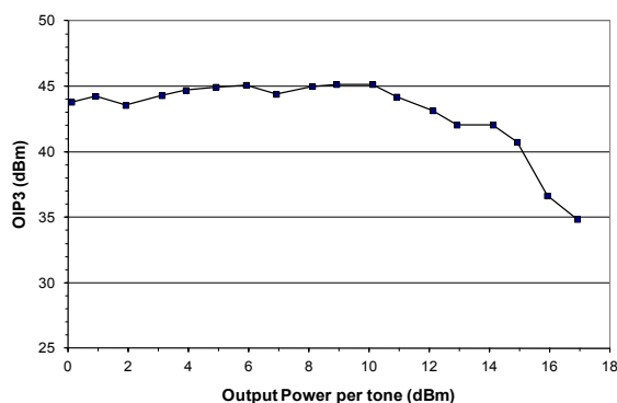
Figure 29: Output 3rd-Order Intercept vs. Power (V SUPPLY = +9 VDC, 2500 MHz Application Circuit)
