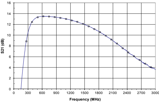
Figure 15: Gain vs. Frequency
