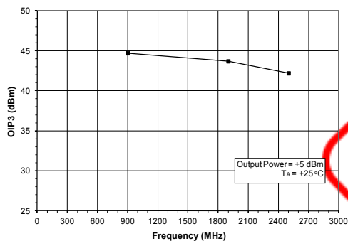
Figure 4: OIP3 vs. Frequency (in Unmatched 50\Omega Test Circuit)
