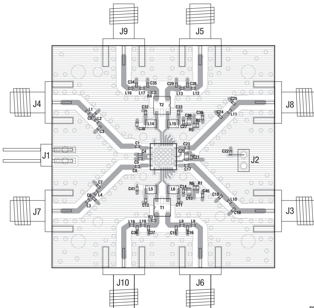
Figure 3. SKY73025-31 Evaluation Board Assembly Diagram
