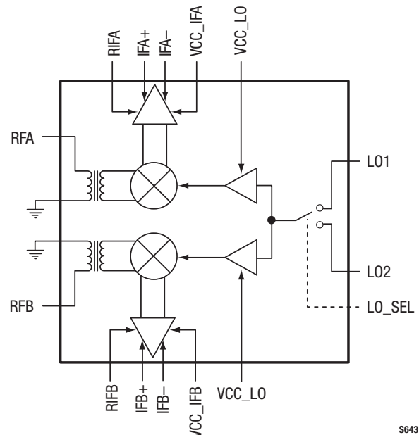
Figure 1. SKY73025-31 Block Diagram
