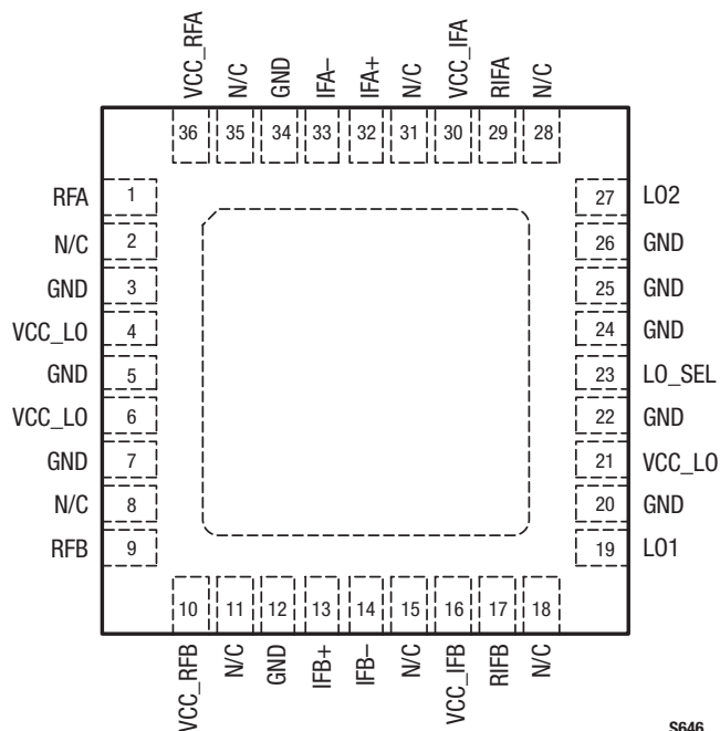
Figure 2. SKY73025-31 Pinout – 36-Pin MCM (Top View)
