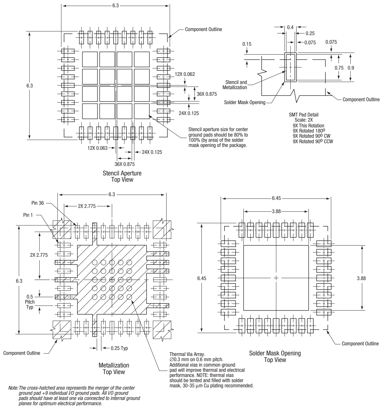
Figure 6. PCB Layout Footprint for the SKY73025-31 6 x 6 mm MCM
