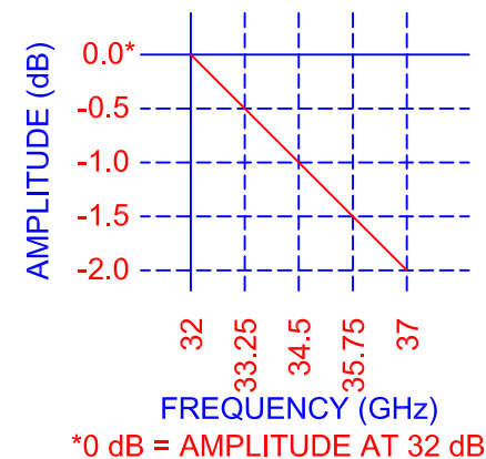
AMPLITUDE VS. FREQUENCY
