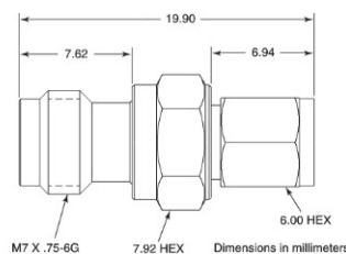
34WVF50 outline
