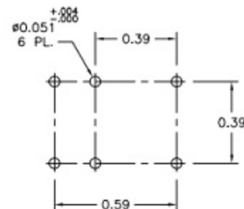
MOUNTING HOLES
