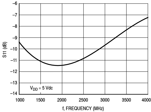
Figure 19. S11 versus Frequency
