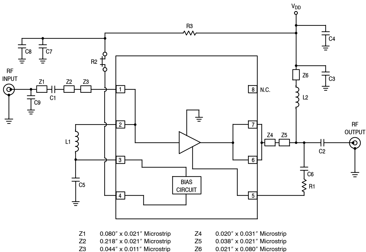
Figure 2. MML20211HT1 Test Circuit Schematic
