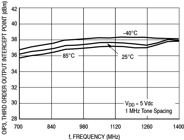
Figure 9. Third Order Output Intercept Point (Two-Tone) versus Frequency versus Temperature
