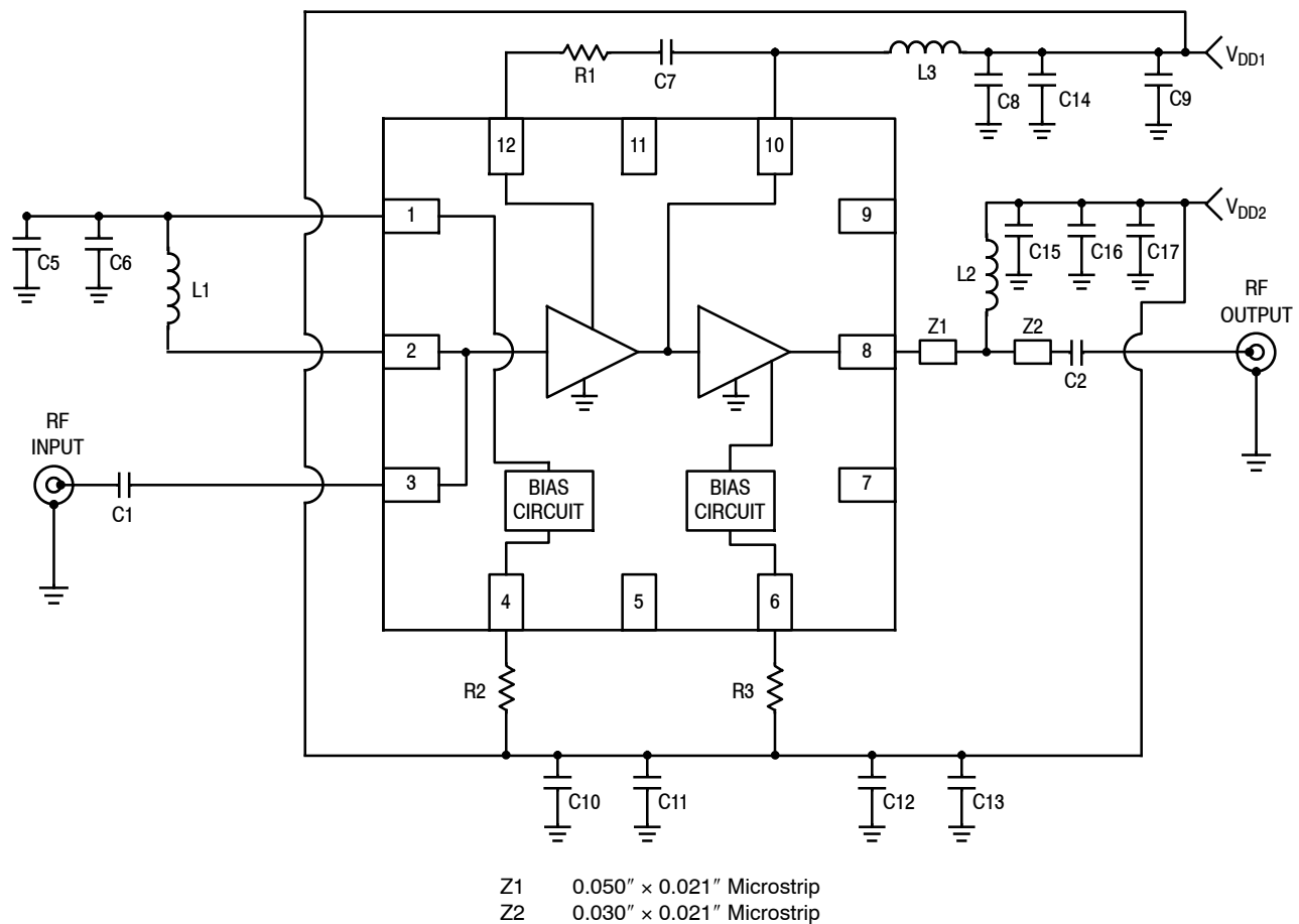
Figure A-3. MML09212HT1 Test Circuit Component Layout
