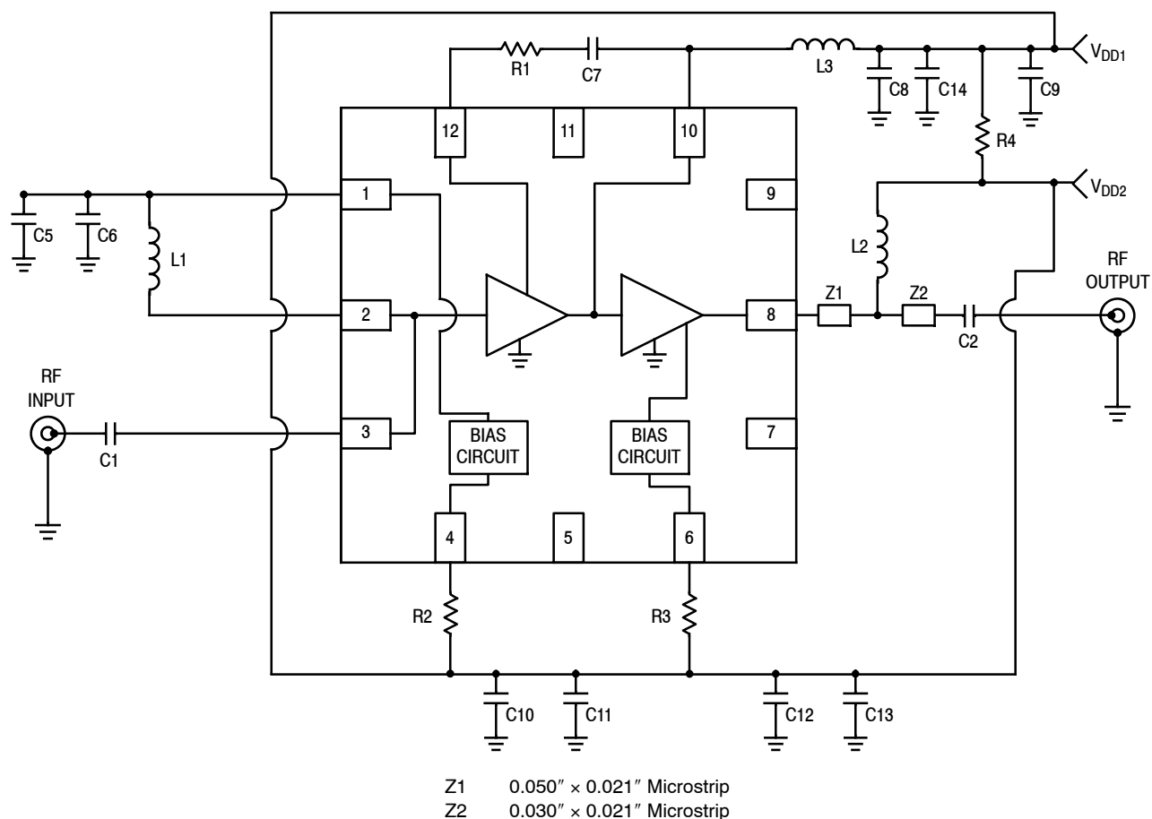
Figure 3. MML09212HT1 Test Circuit Schematic
