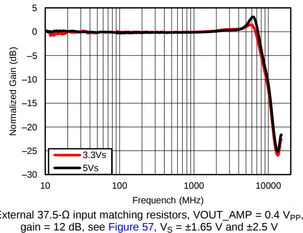
Figure 2. Frequency Response Differential Input
