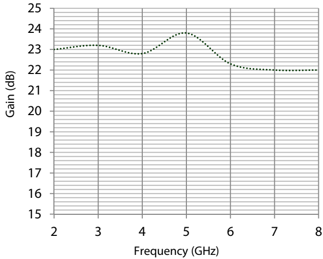
Gain (dB)
