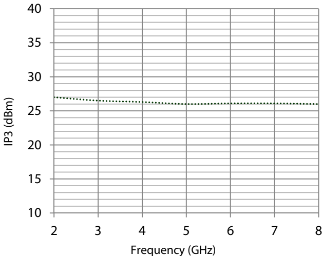
3 rd Order Intercept (dBm)
