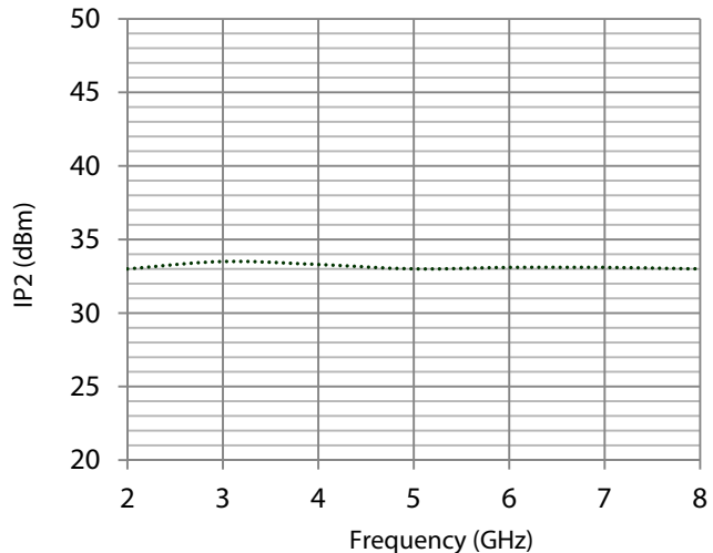
2 nd Order Intercept (dBm)
