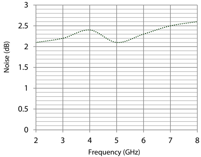
Noise Figure (dB)
