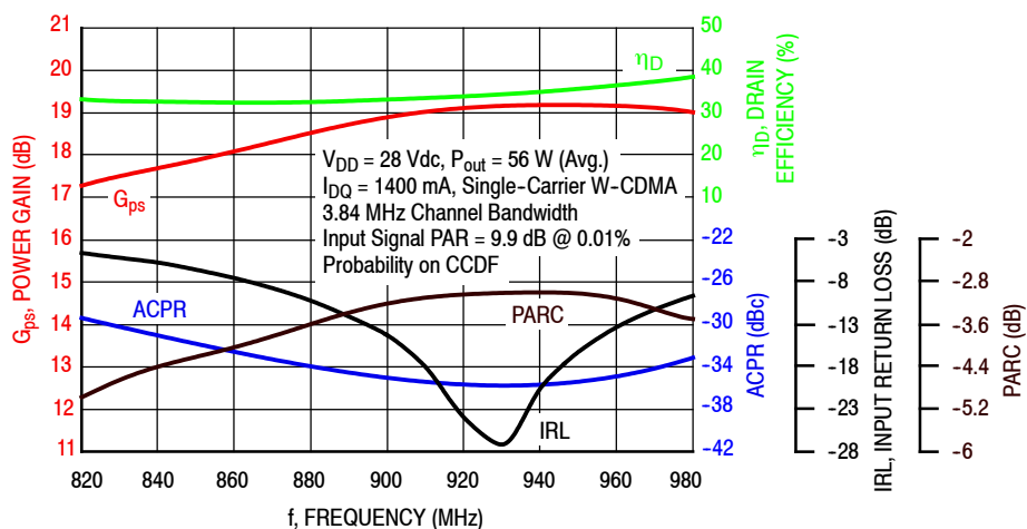
Figure 3. Single-Carrier Output Peak-to-Average Ratio Compression (PARC) Broadband Performance @ P_{out} = 56 \text{ Watts Avg.}
