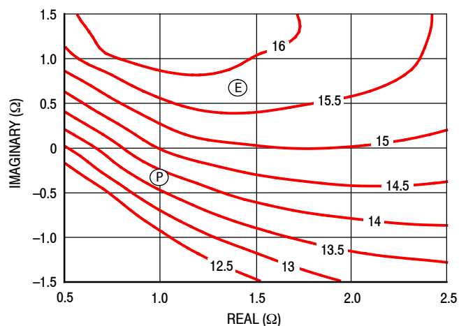
Figure 42. P3dB Load Pull Gain Contours (dB)
