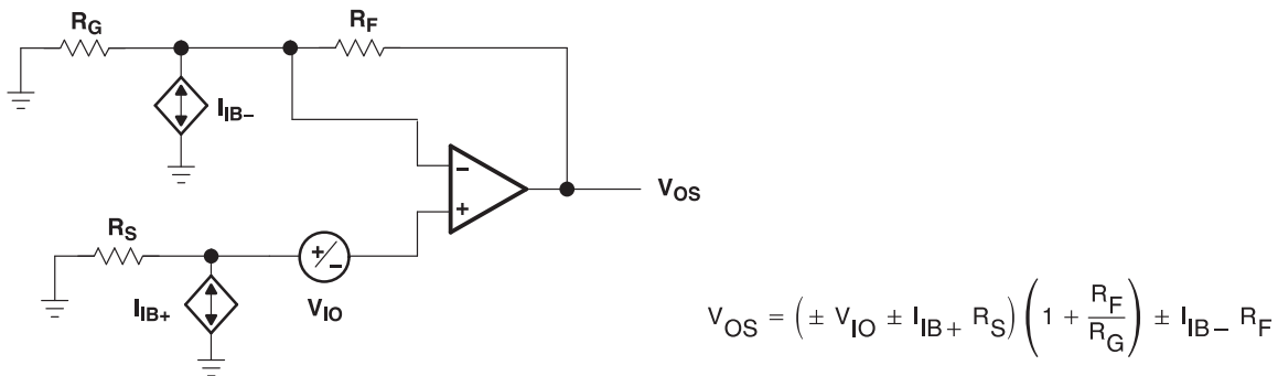
Figure 46. Output Offset Voltage Model
