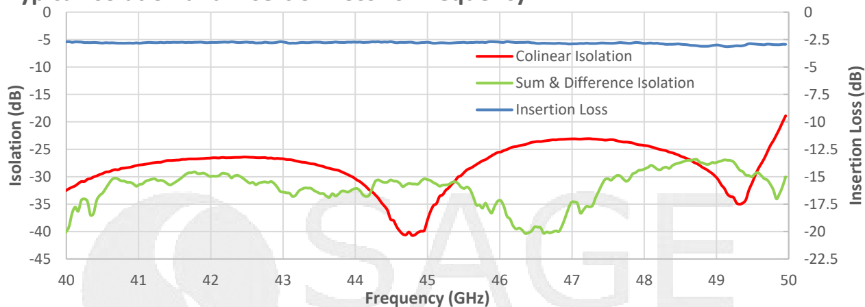
Typical Isolation and Insertion Loss vs. Frequency
