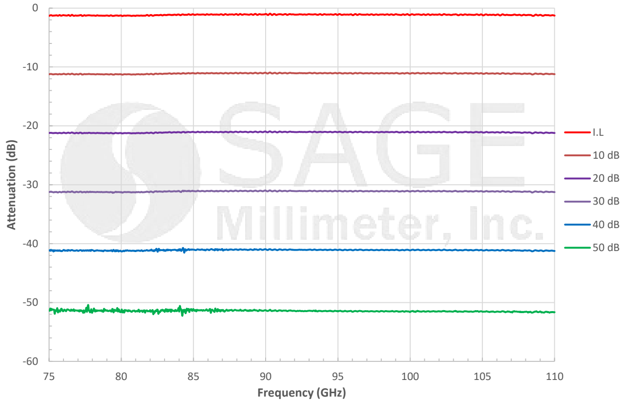
Typical Attenuation vs. Frequency
