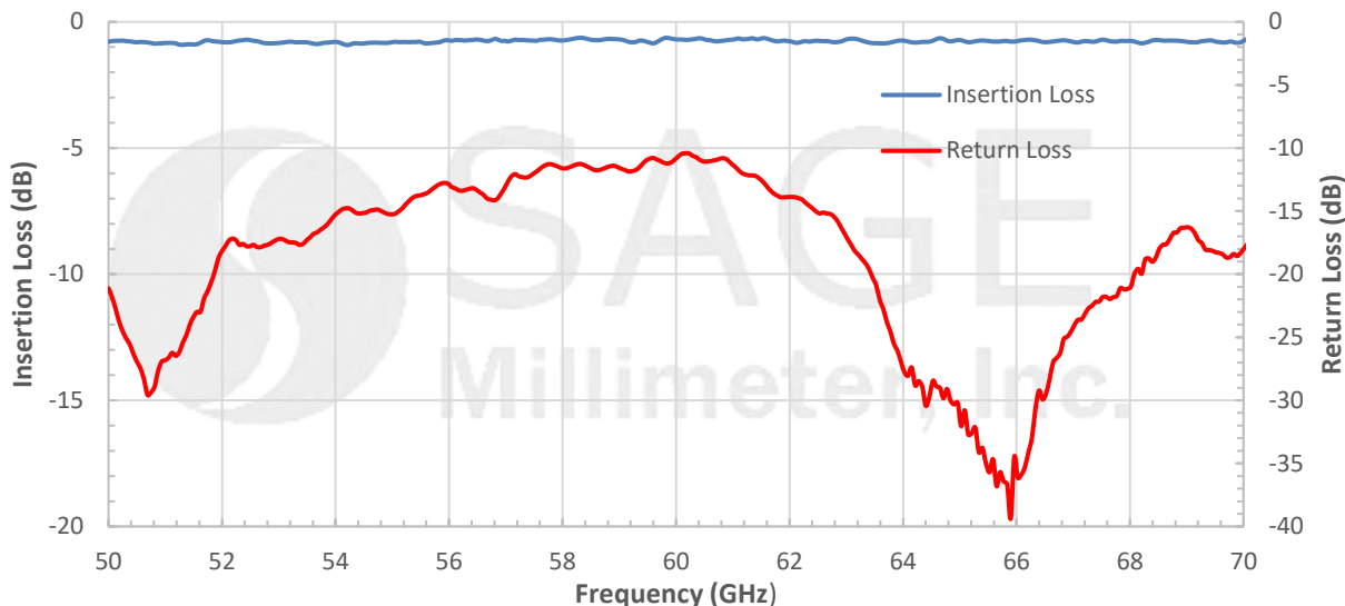
Typical Insertion Loss and Return Loss vs. Frequency (Back to Back)
