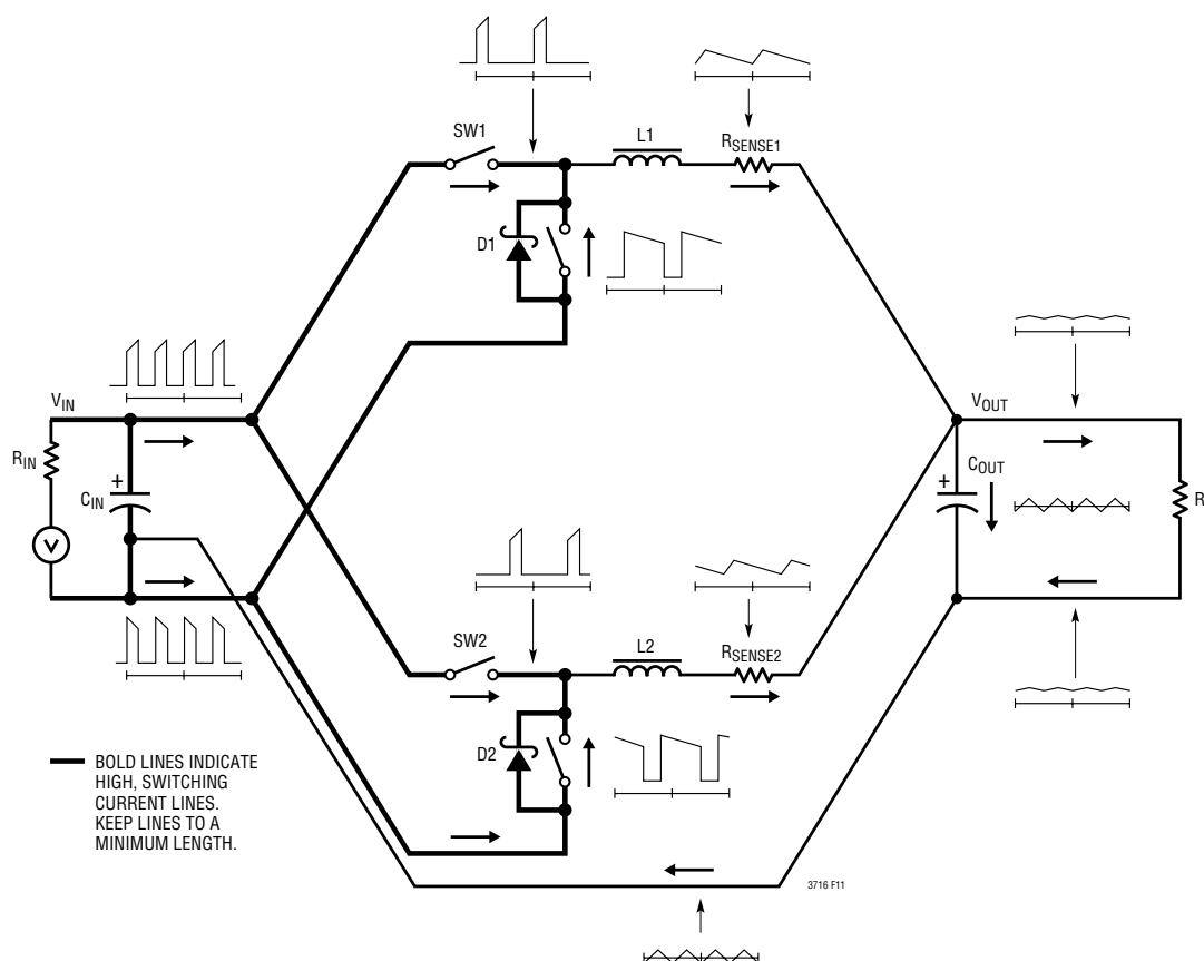
Figure 11. Instantaneous Current Path Flow in a Multiple Phase Switching Regulator
