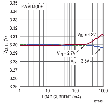
Buck-Boost Regulator, Load Regulation
