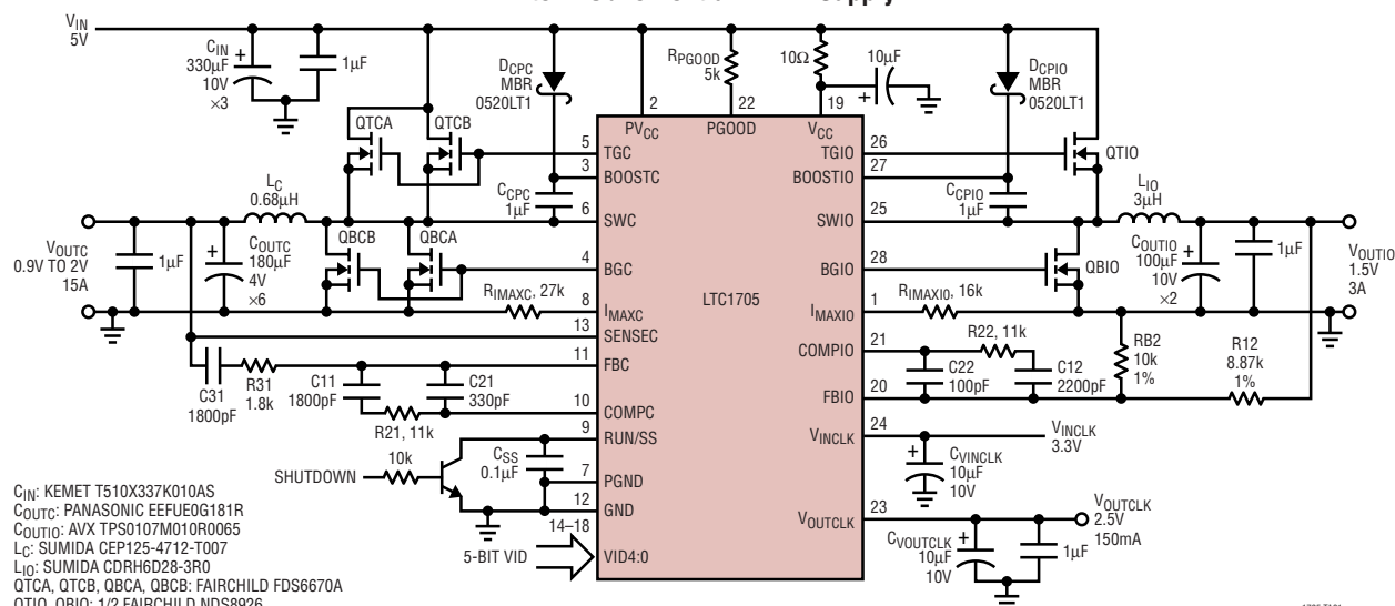
Intel Mobile Pentium VRM Supply
