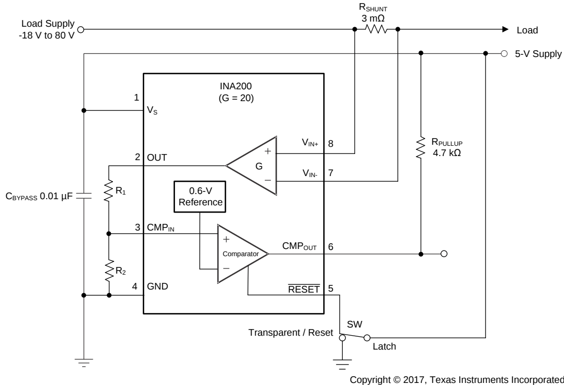
图 26. INA200 Basic Connections
