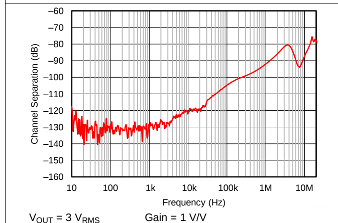
图 11. Channel Separation vs Frequency
