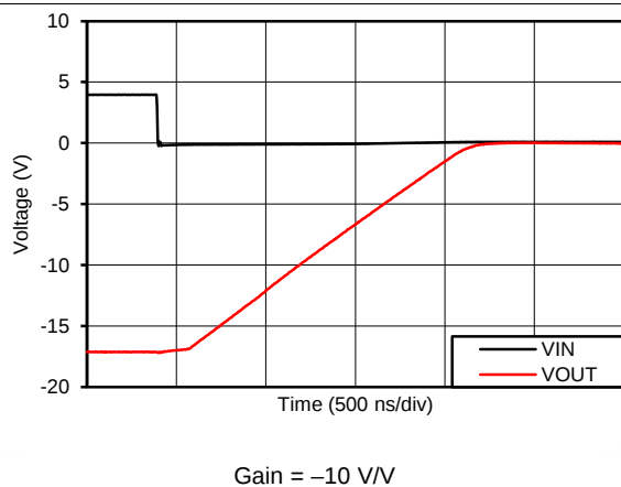
图 27. Negative Overload Recovery
