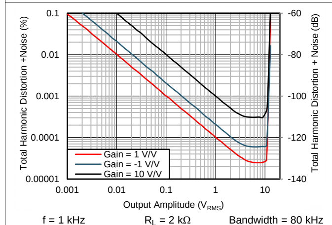
图 9. THD+N Ratio vs Output Amplitude
