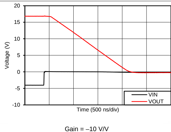
图 28. Positive Overload Recovery
