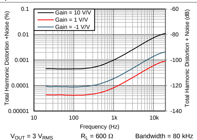
图 8. THD+N Ratio vs Frequency
