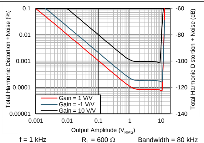
图 10. THD+N Ratio vs Output Amplitude
