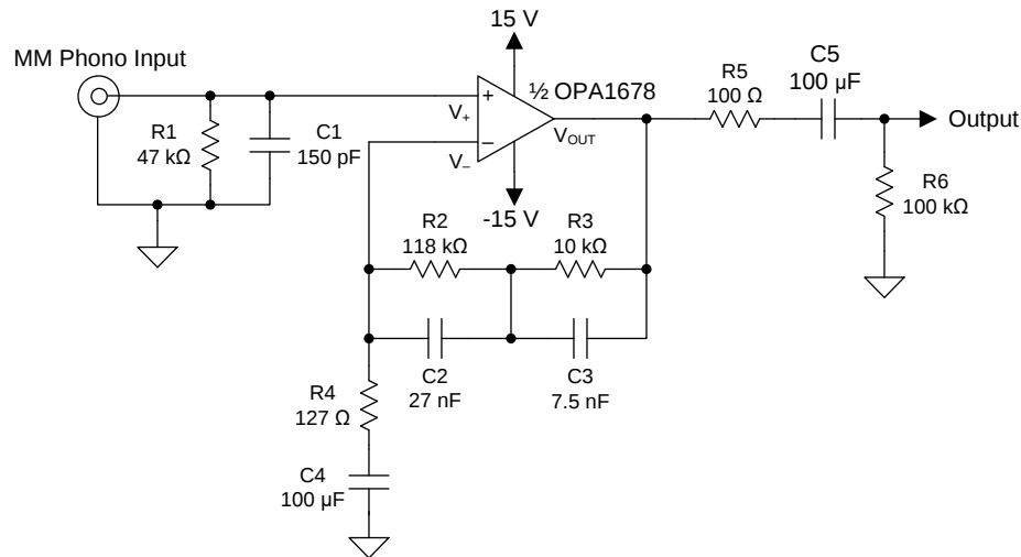
图 38. Phono Preamplifier for Moving Magnet Cartridges (Single-Channel Shown)
