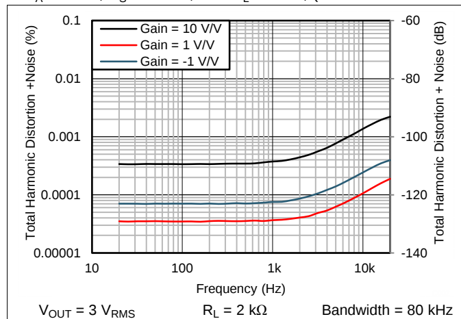
图 7. THD+N Ratio vs Frequency
