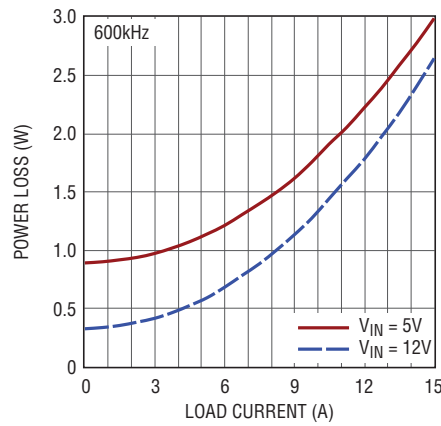
Figure 10. Power Loss at 1.5V Output
