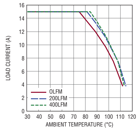
Figure 14. 5V to 1.5V Derating Curve, No Heat Sink
