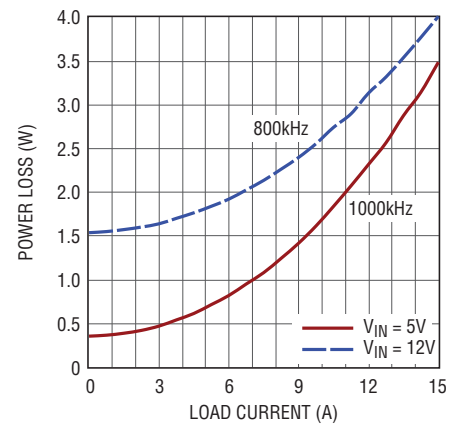
Figure 11. Power Loss at 3.3V Output
