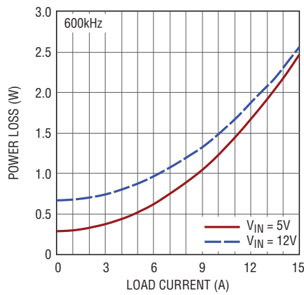
Figure 9. Power Loss at 1V Output
