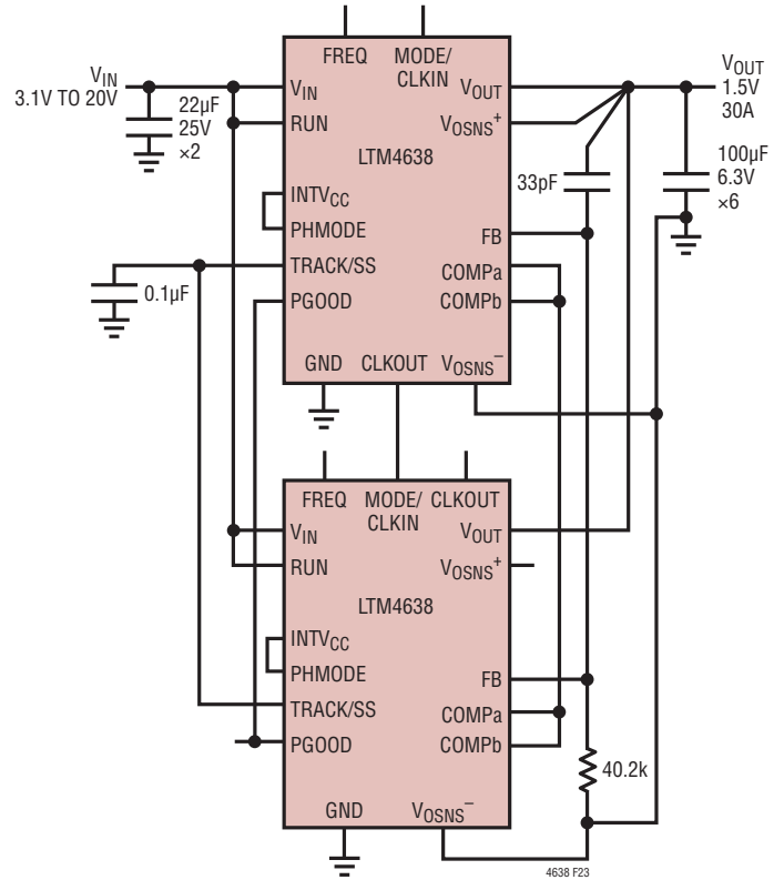
Figure 23. 3.1V IN to 20V IN , Two Phases, 1.5V at 30A Design
