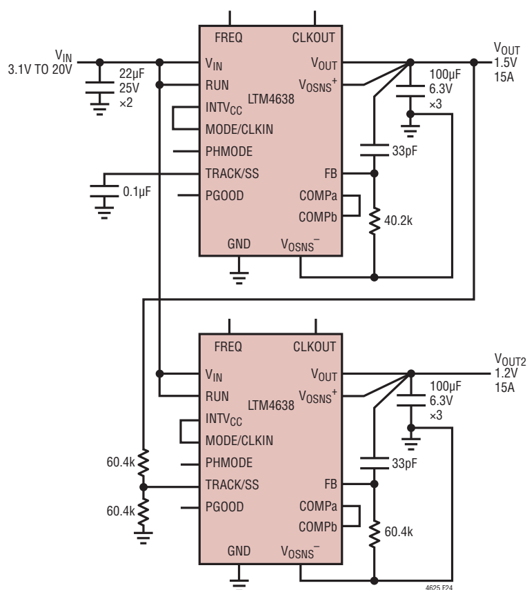
Figure 24. 3.1V IN to 20V IN , 1.2V and 1.5V with Coincident Tracking
