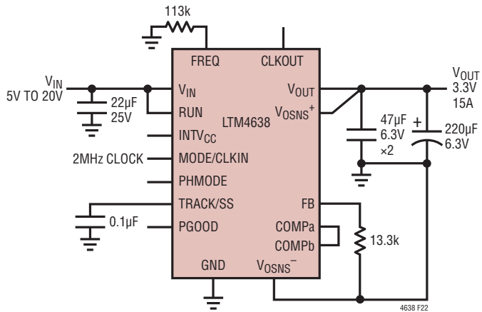
Figure 22. 5V IN to 20V IN , 3.3V Output with 2MHz External Clock
