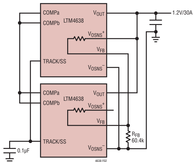
Figure 2. 4-Phase Parallel Configurations
