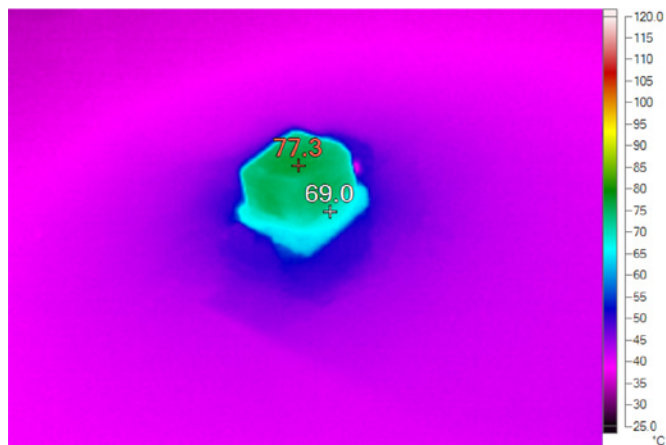
Figure 19. Thermal Image at 12V Input, 1.0V Output Without Air Flow and Heat Sinking
