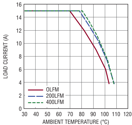
Figure 15. 12V to 1.5V Derating Curve, No Heat Sink
