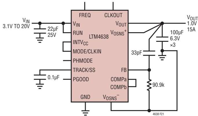
Figure 21. 3.1V IN to 20V IN , 1V Output at 15A Design
