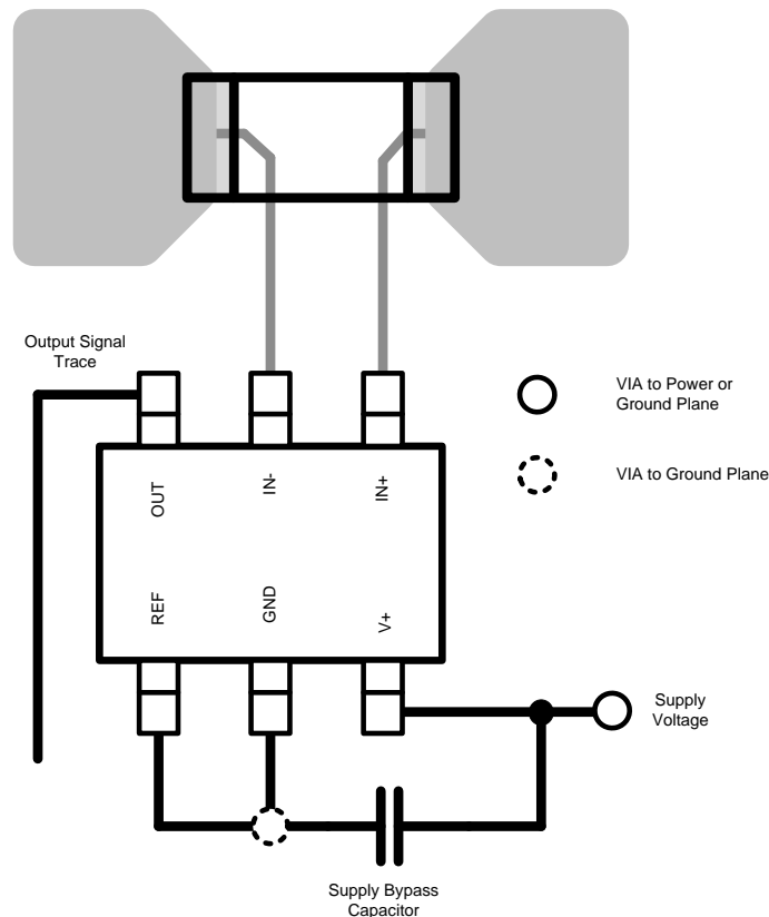
图 34. Recommended Layout
