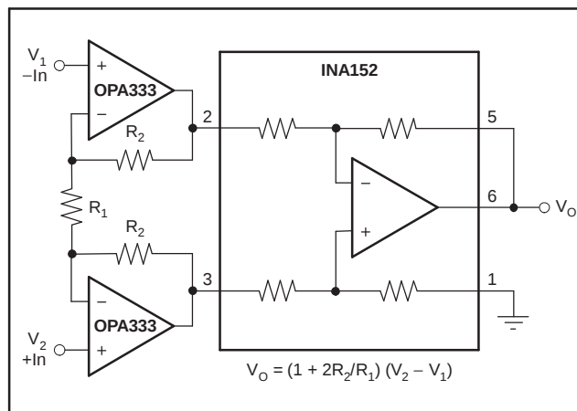
Figure 8. Precision Instrumentation Amplifier
