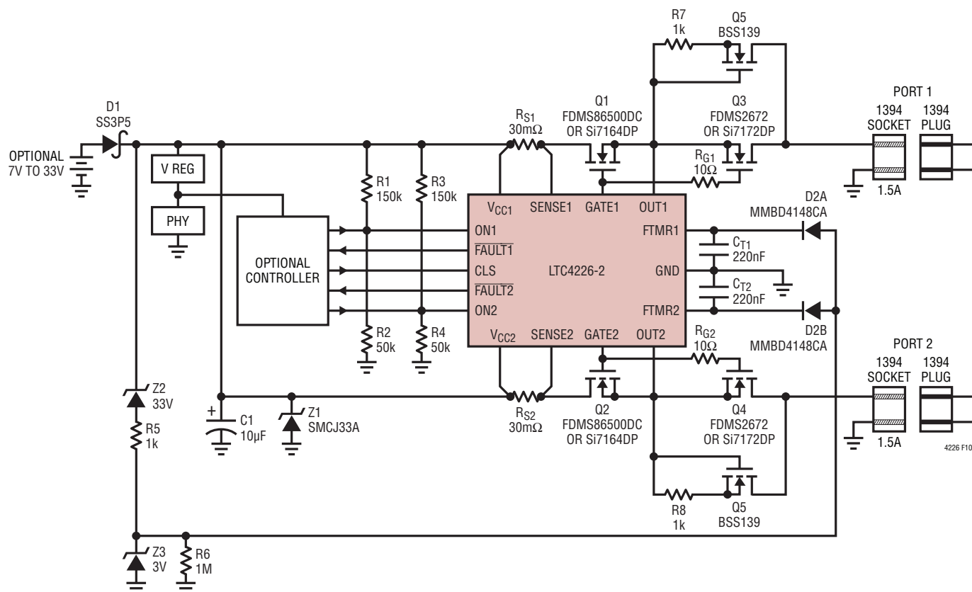
Figure 10. 2 FireWire Ports with Positive Overvoltage Isolation
