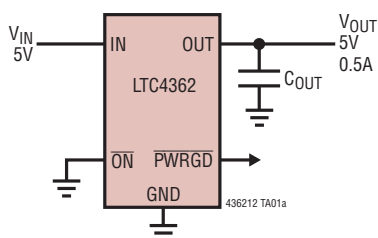
Protection from Overvoltage and Overcurrent
