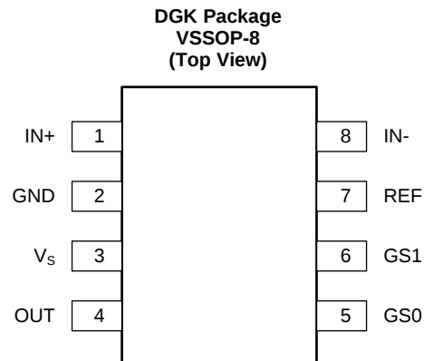
Pin Functions
