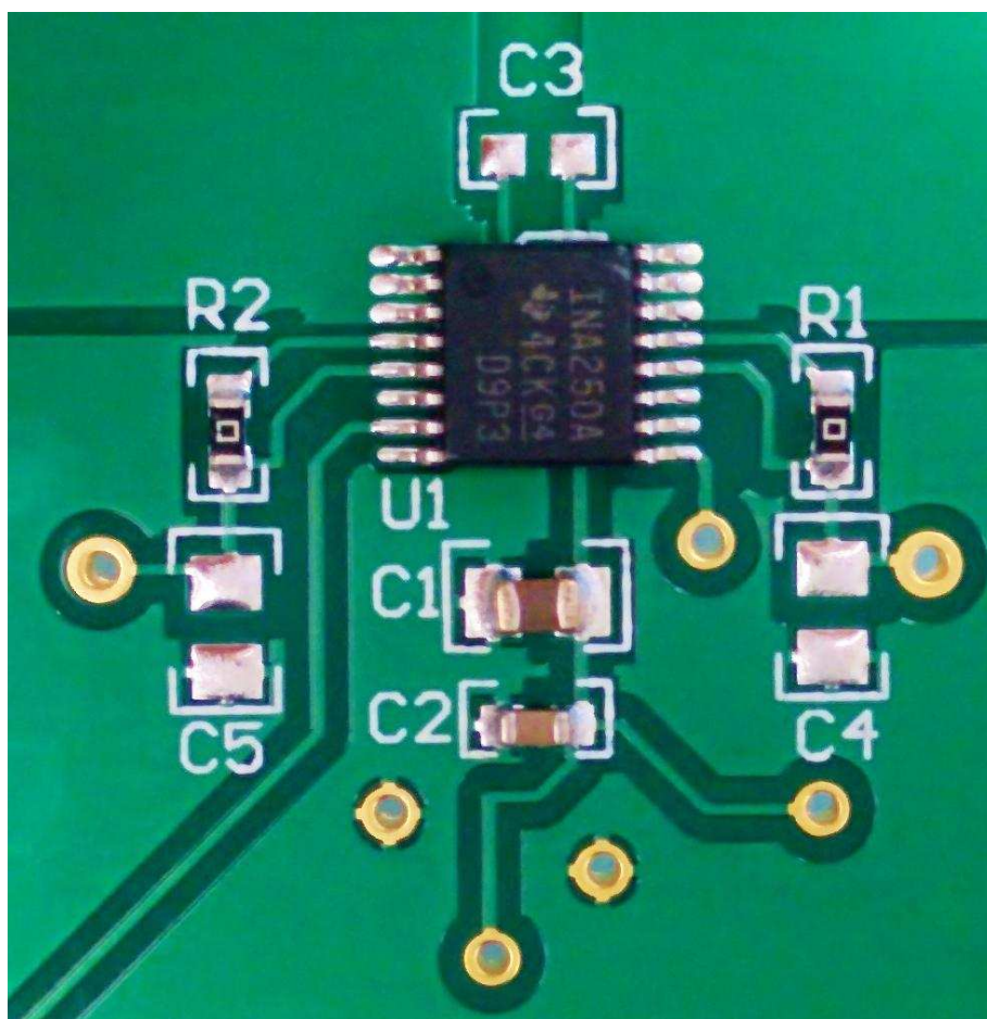
Figure 43. Recommended Layout
