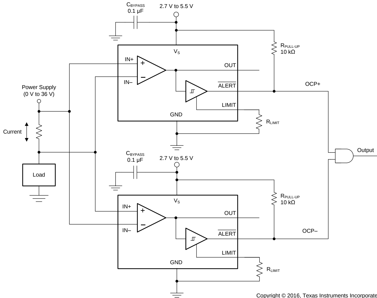
图 42. Bidirectional Application
