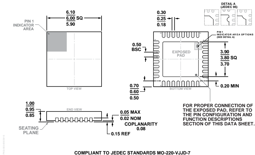
COMPLIANT TO JEDEC STANDARDS MO-220-VJJD-7 Figure 4. 32-Lead Lead Frame Chip Scale Package [LFCS] 6 mm × 6 mm Body and 0.95 mm Package Height (CP-32-15) Dimensions shown in millimeters
