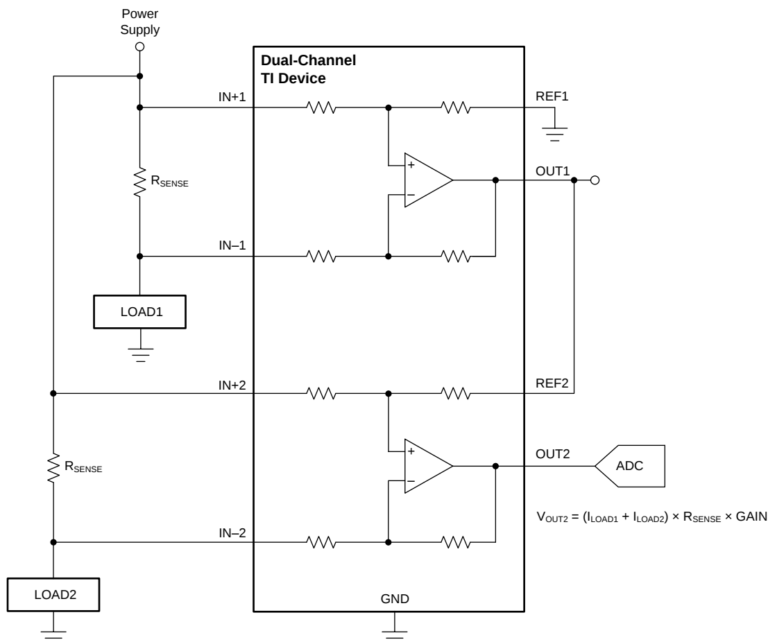
图 49. Summing Multiple Currents
