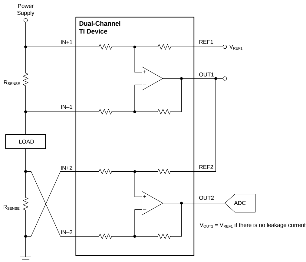
图 51. Detecting Leakage Currents
