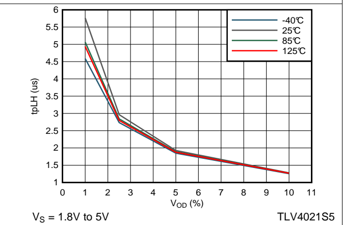
Figure 30. Propagation Delay Low-High vs Input Overdrive
