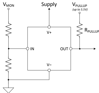
Figure 44. Level-Shifting
