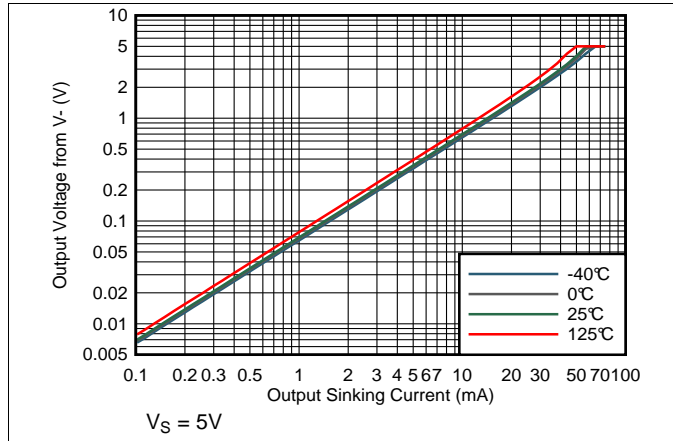
Figure 27. Output Voltage vs Output Sinking Current
