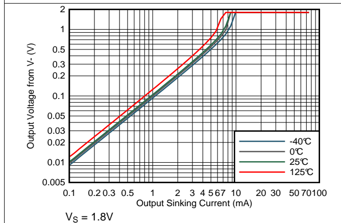
Figure 23. Output Voltage vs Output Sinking Current
