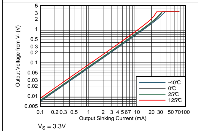
Figure 25. Output Voltage vs Output Sinking Current
