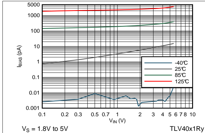
Figure 21. Bias Current vs Common Mode Voltage
