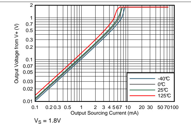
Figure 24. Output Voltage vs Output Sourcing Current
