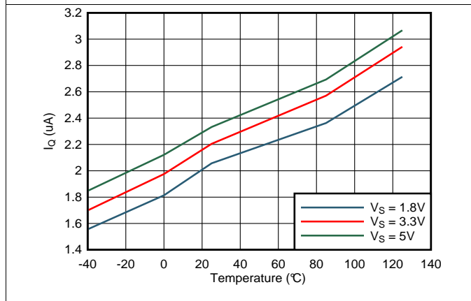
Figure 29. Supply Current vs Temperature
