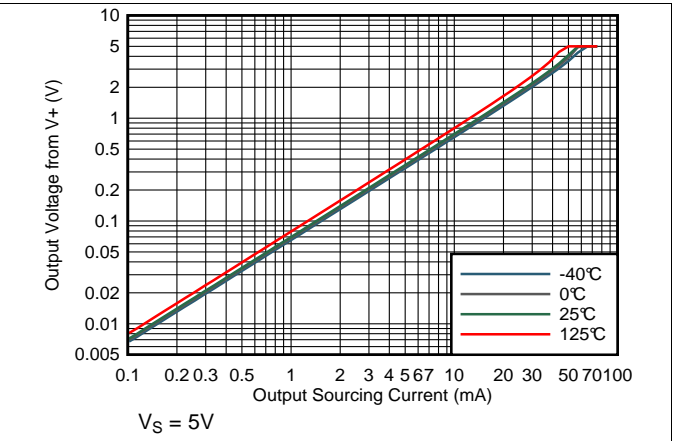
Figure 28. Output Voltage vs Output Sourcing Current
