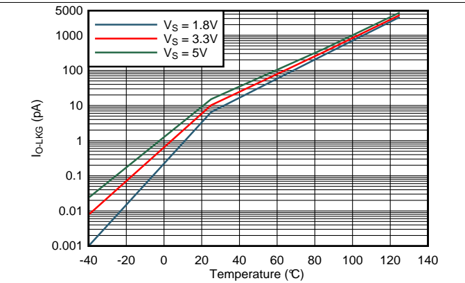
Figure 22. Output Current Leakage vs Temperature
