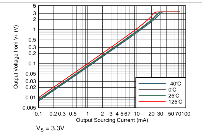
Figure 26. Output Voltage vs Output Sourcing Current
