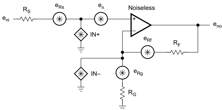
Figure 51. Noise Model
