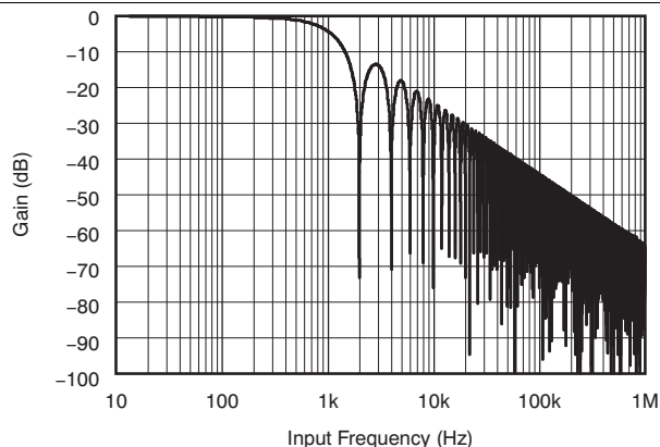
Figure 1. Frequency Response
