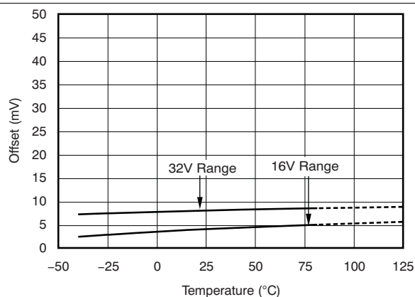
Figure 2. ADC Shunt Offset vs Temperature
