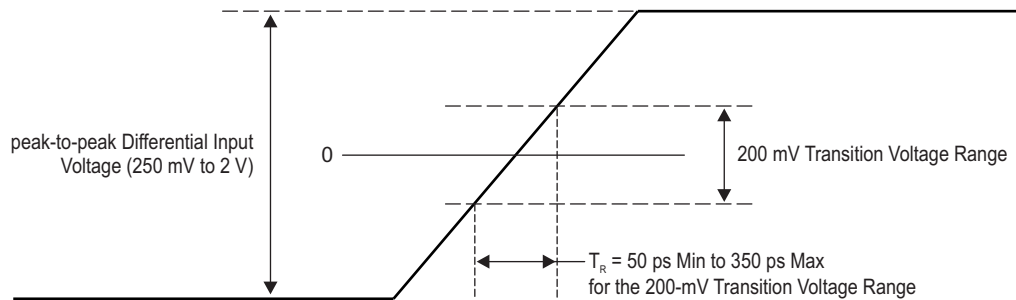
图 11-20. CORECLK, SGMII0CLK and USBCLK Clock Transition Time
