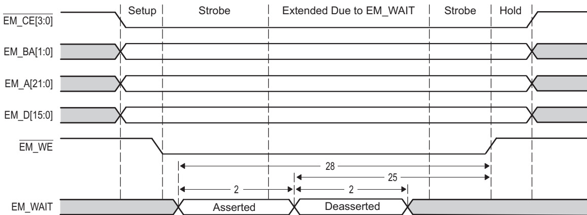
图 11-55. EMIF16 EM_WAIT Write Timing Diagram
