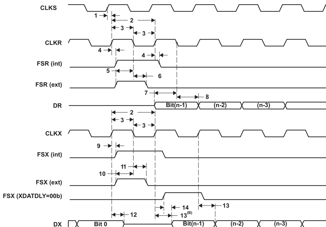
Figure 5-25. McBSP Timing
