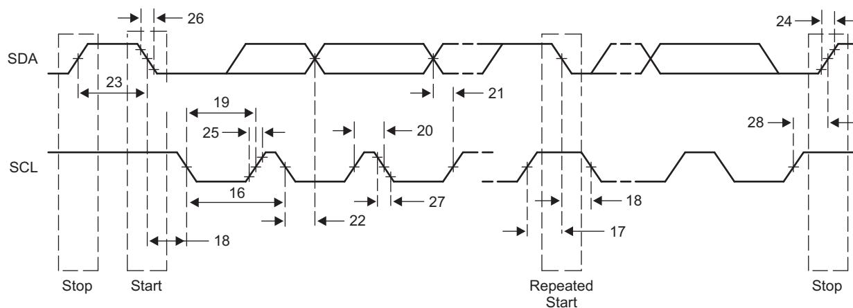
Figure 5-10. I 2 C Transmit Timings
