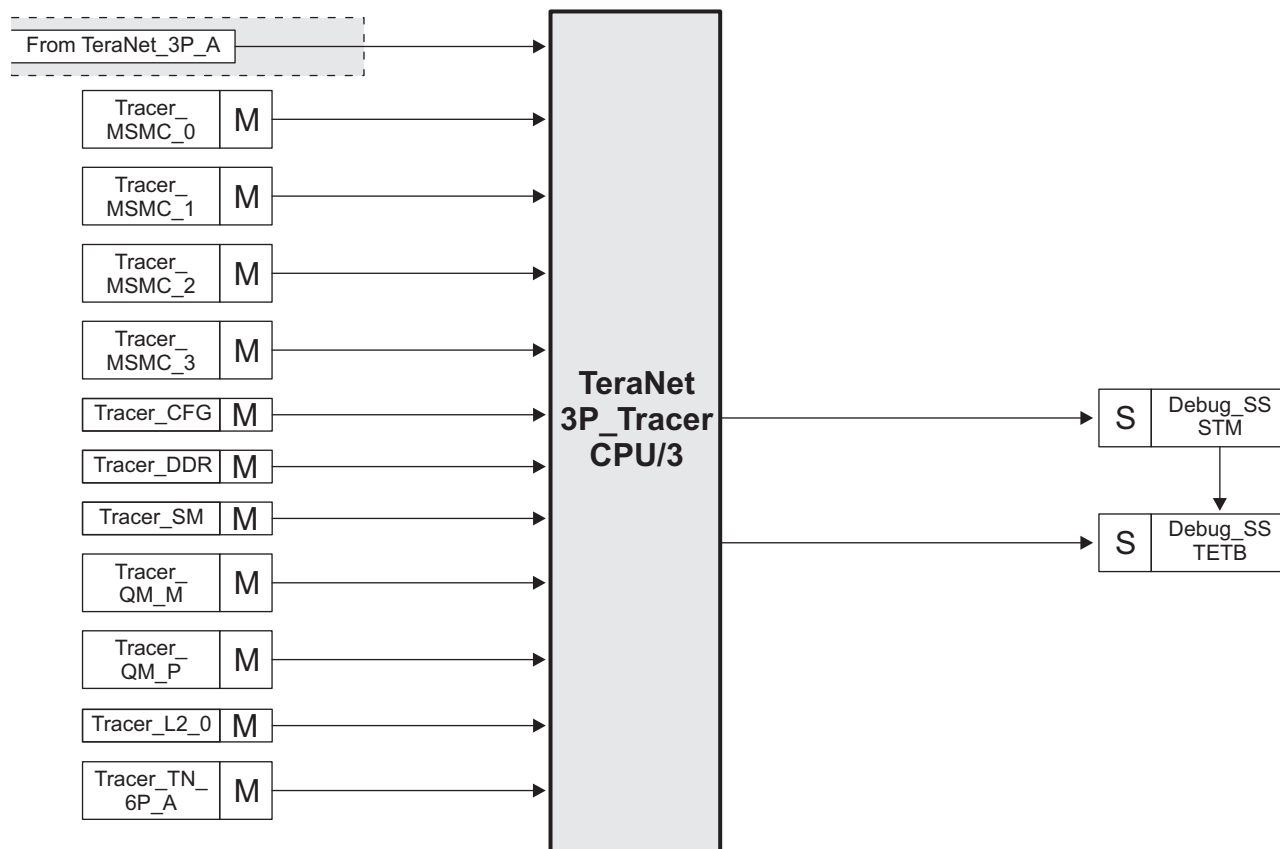
Figure 9-4. TeraNet 3P_Tracer
