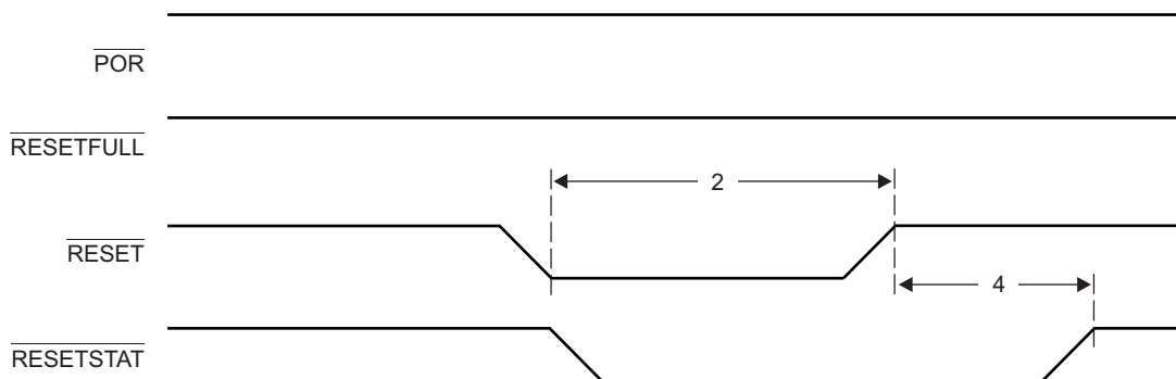
Figure 5-3. Soft/Hard-Reset Timing
