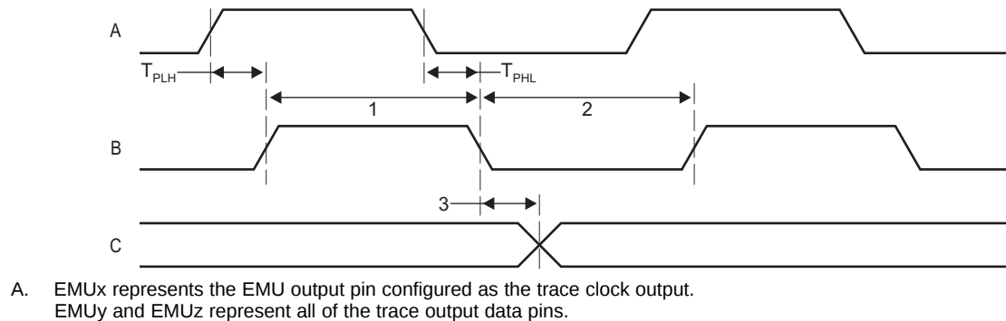
Figure 5-31. Trace Timing
