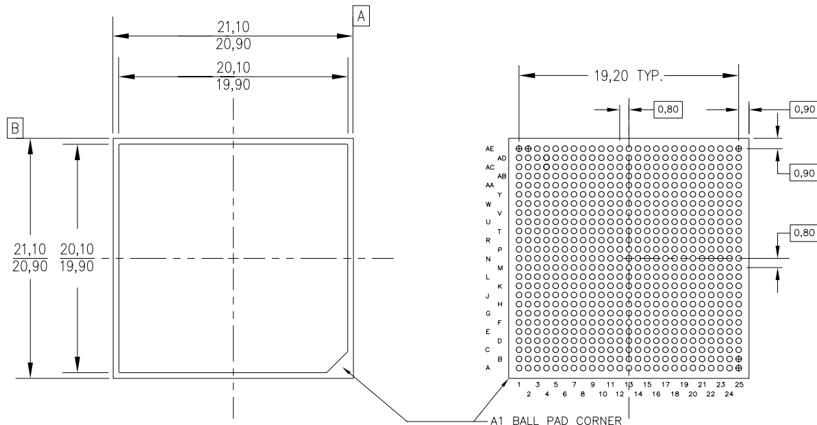
Bottom View
