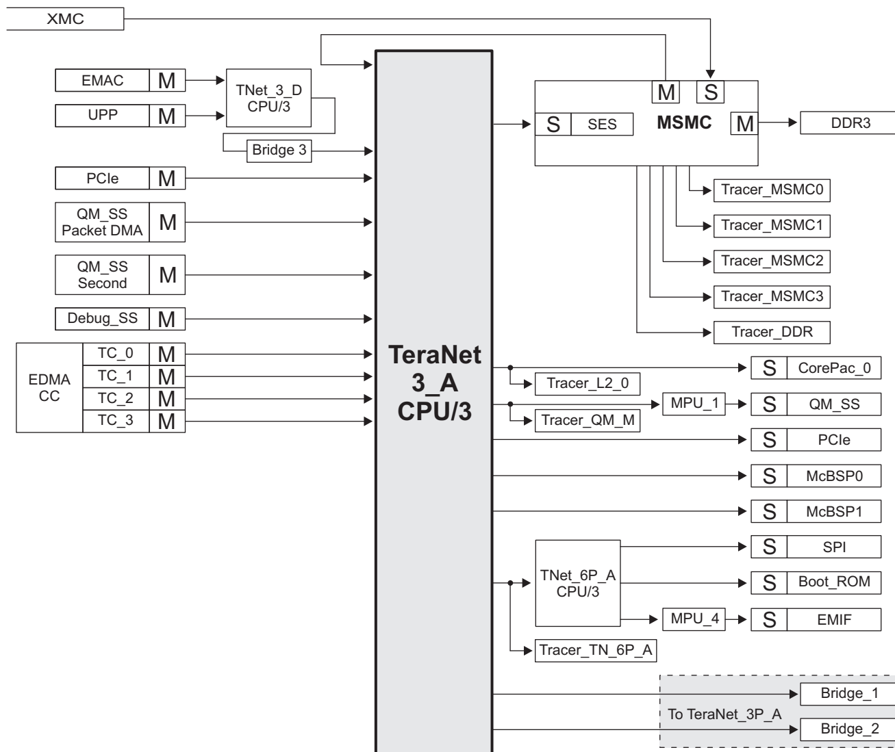
Figure 9-1. TeraNet 3A
