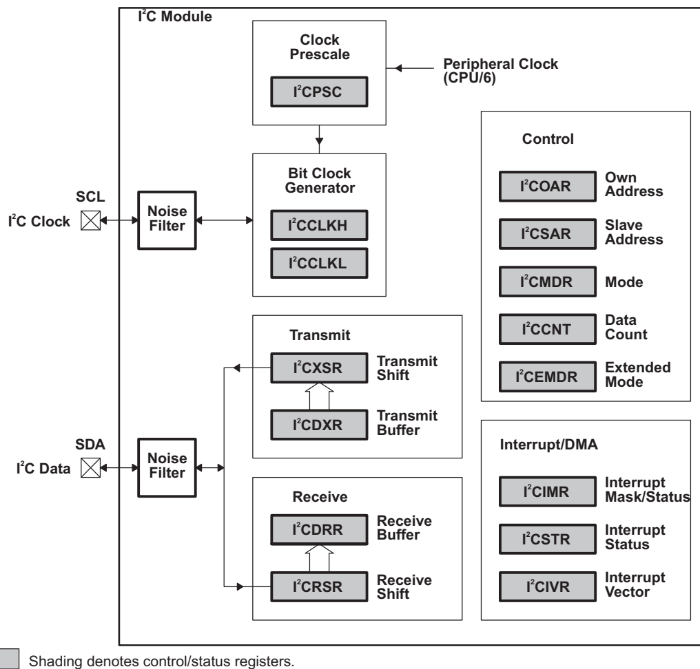
Figure 6-23. I²C Module Block Diagram
