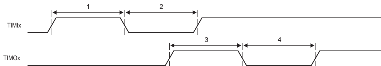
Figure 5-23. Timer Timing
