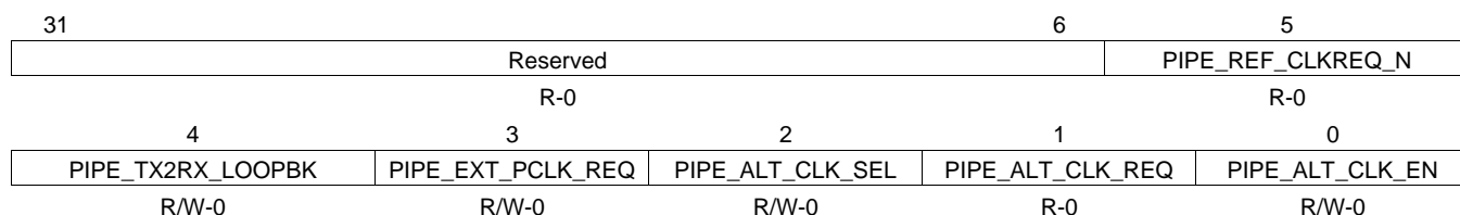
图 8-35. USB_PHY_CTL1 Register
