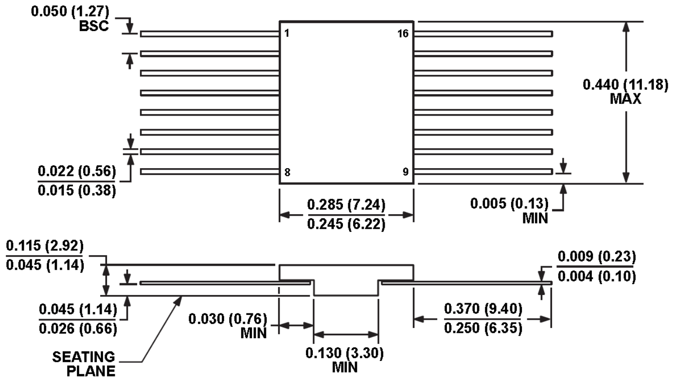
Figure 10. 16-Lead Bottom Brazed Flatpack
