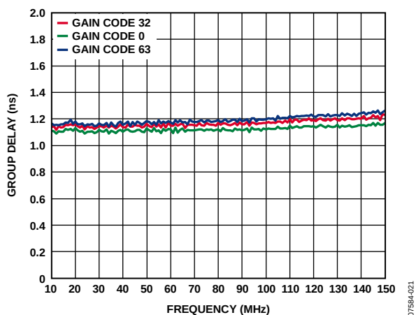
Figure 36. Group Delay vs. Frequency at Gain Code 0, Gain Code 32, and Gain Code 63
