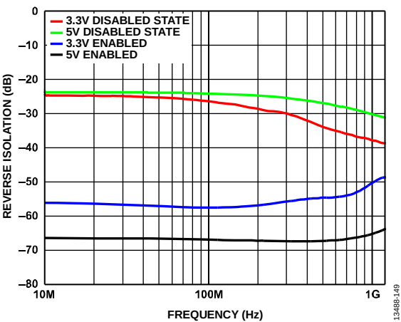
Figure 48. Reverse Isolation vs. Frequency
