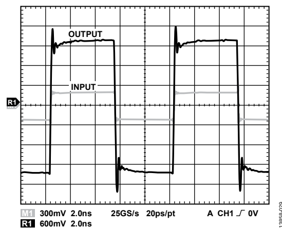
Figure 30. Large Signal Pulse Response, V_{OUT} = 4\text{ V p-p} , V_S = 3.3\text{ V}
