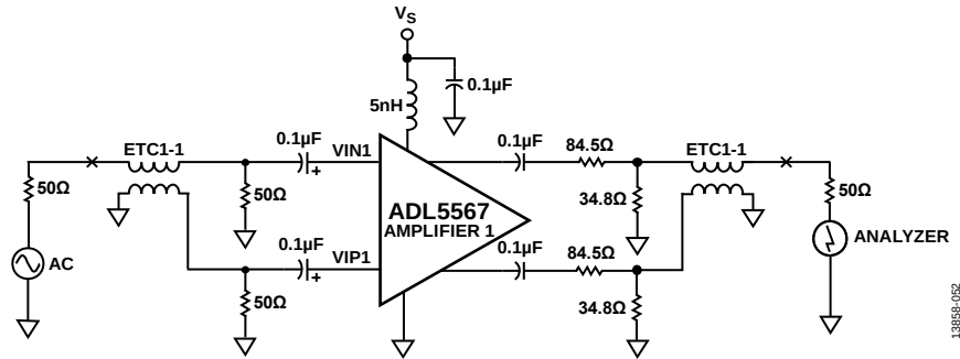
Figure 52. General-Purpose Characterization Circuit
