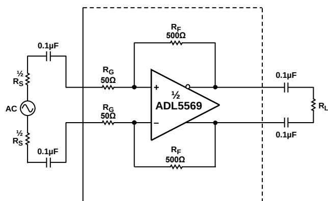
Figure 38. Basic Structure
