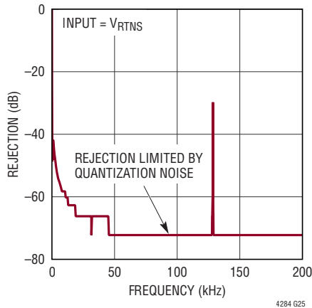
12-Bit ADC Input Signal Attenuation (Calculated, Extended Frequencies)
