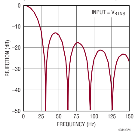
12-Bit ADC Input Signal Attenuation (Calculated, Low Frequencies)
